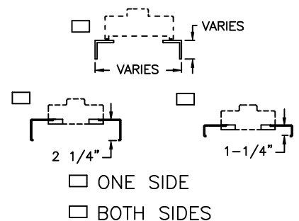
UNITIZED DOOR SYSTEM SHOWN CHEM-PRUF® EXCLUSIVE UP TO 32 SQ. FT.
