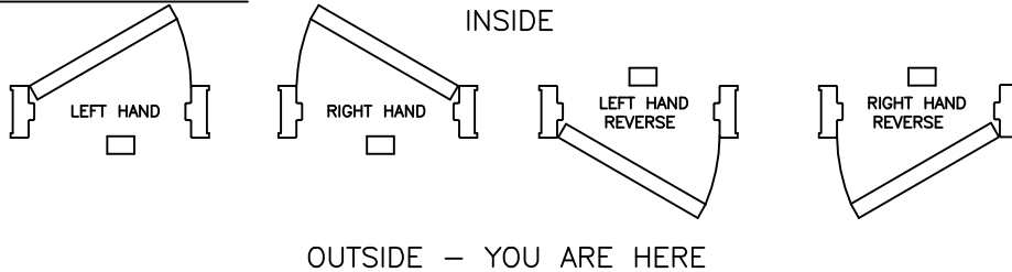
UNITIZED DOOR SYSTEM SHOWN CHEM-PRUF® EXCLUSIVE UP TO 32 SQ. FT.
